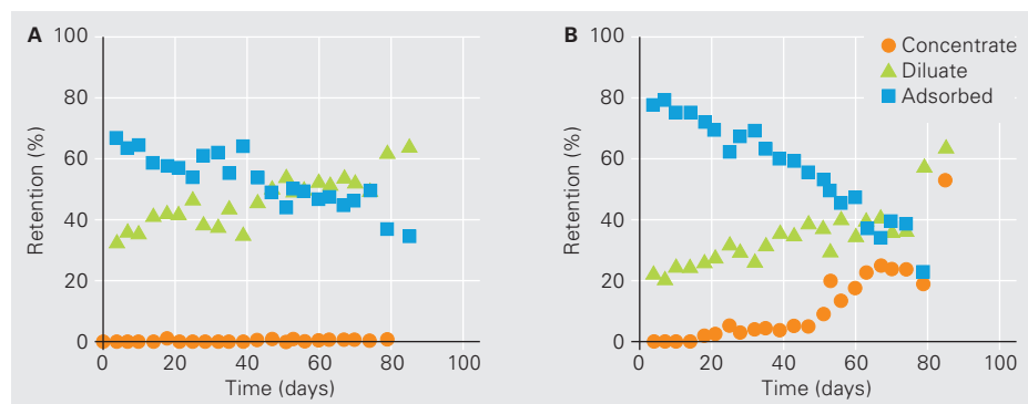
Fig. 3: Mass balances of ethinyl estradiol (A) and propranolol (B) in electro dialysis.
